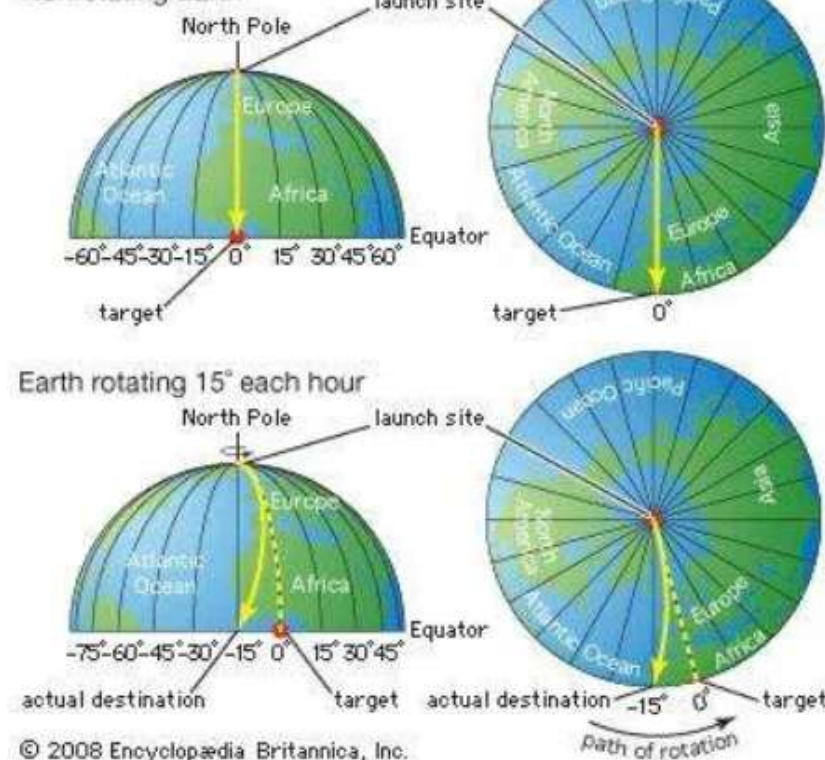
The effect of the Coriolis force
