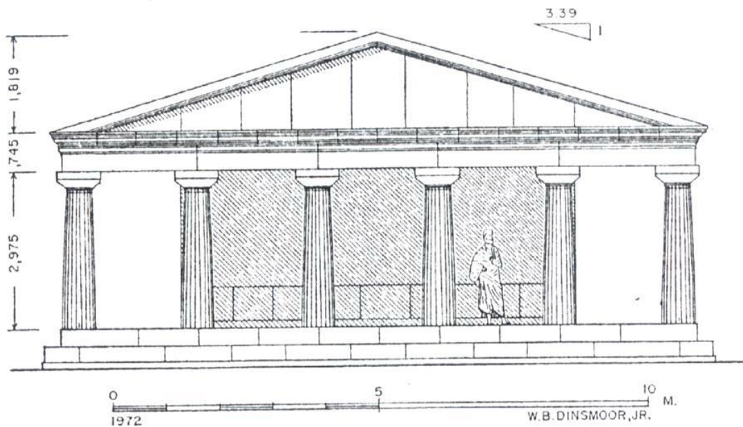
Abb. 1. Restored Rear Elevation
