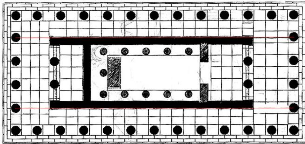
FIG. 67.—THE ΗΗΡΗΑΕΣΤΕΙΟΝ. (Restored by Dinsmoor.)
