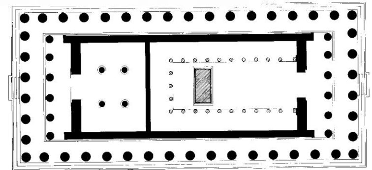
564 Above: the Older Parthenon, 488-480 B.C. Centre: the Parthenon, 447-438 B.C. Below: the
