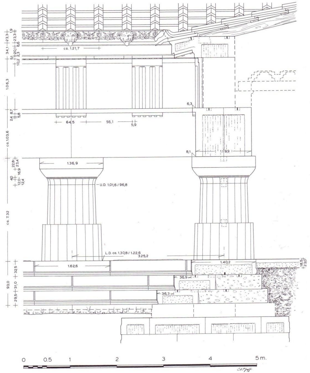
FIGURE 54. RESTORATION OF THE ORDER OF THE FLANK PTEROMA
