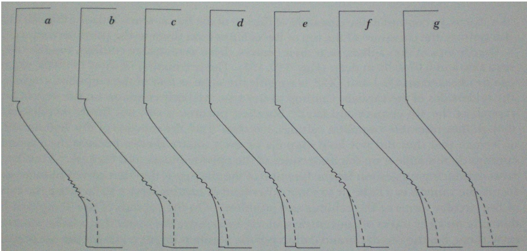
FIGURE 60. COMPARISON OF THE PROFILES OF DORIC CAPITALS ( not to scale ): a. Parthenon, Athens; b. Hephaisteion, Athens; c. Temple of Hera, Argive Heraion; d. Tholos, Delphi; e. Temple of Asklepios, Epidaurus; f. Temple of Athena Alea, Tegea; g. Temple of Zeus, Nemea
