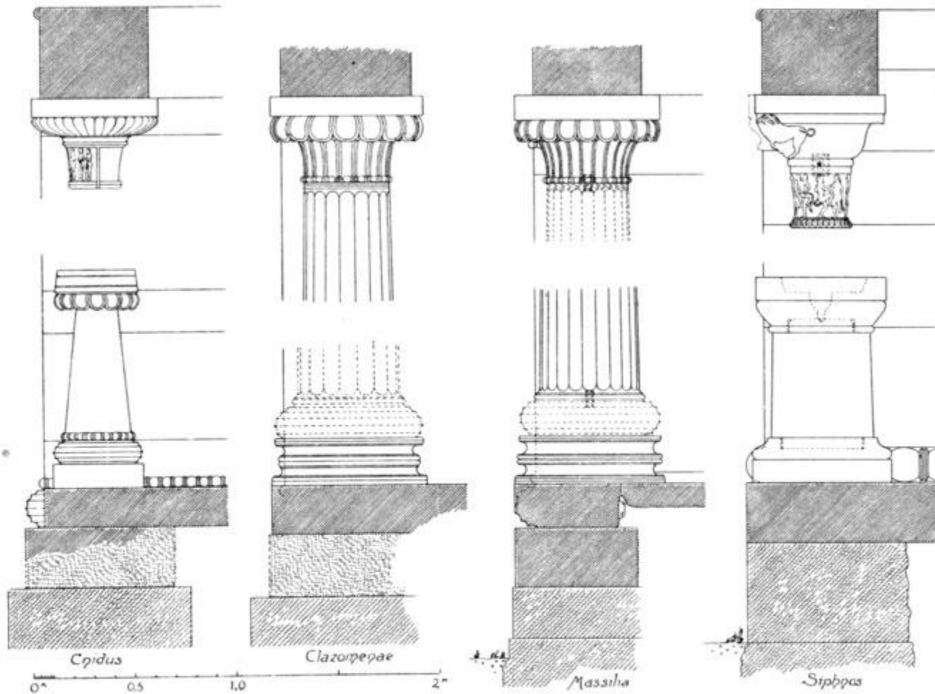
Figure 3. Supports ἐν παραστάσιν .
