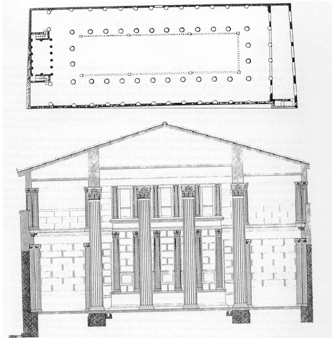
Fig. 3a (top). Basilica, Pompeii, plan (Gros 1996 [supra n.2] fig. 287, after Ohr [supra n.2] pl. 38).
