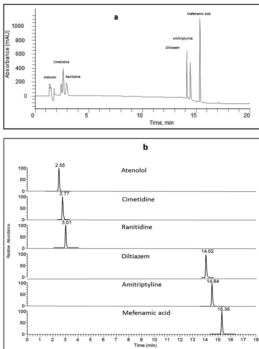
Fig. 1 Chromatogram of a mixture of the pharmaceuticals in MeOH. Chromatographic conditions: Zorbax Eclipse XDB-C18 reverse-phase column (250 mm \times 4 mm i.d., 5 \mu\text{m} ); mobile phase of 10 mM ammonium acetate with acetic acid and ACN at pH = 4.8; flow rate 1.0 \text{ mL min}^{-1} ; (a) at \lambda_{\text{max}} = 225 nm for HPLC; (b) MRM chromatogram for LC-ESI-MS/MS.
