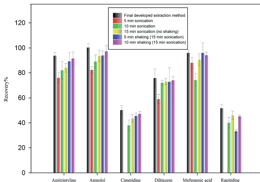
Fig. 2 Recovery of selected pharmaceuticals using the optimized method at different sonication and shaking times (BTC sediment).
