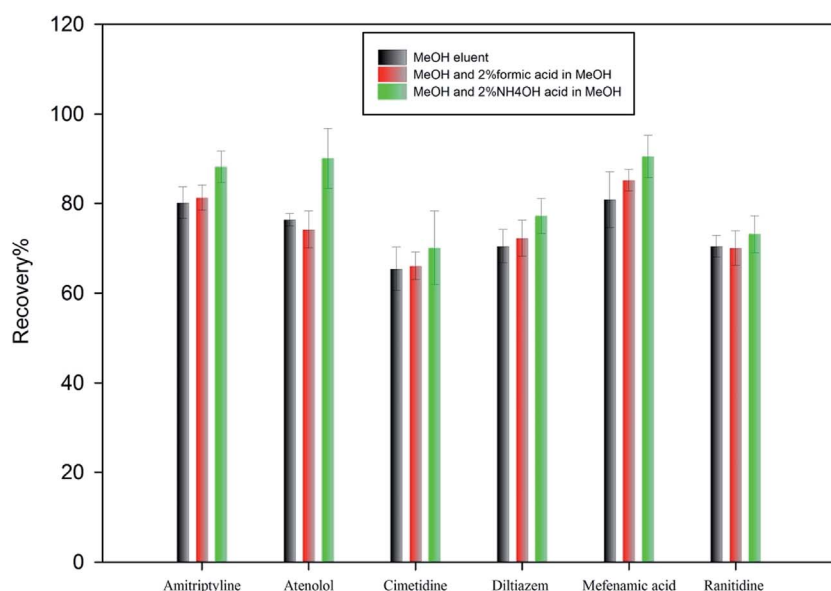
Fig. 3 Total recoveries of selected pharmaceuticals using different SPE elution solvents (BTC sediment).
