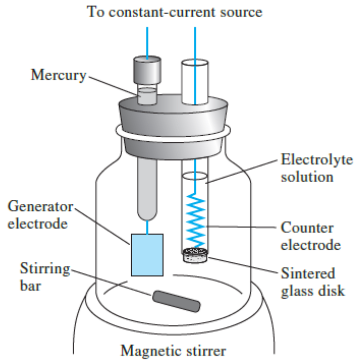
FIGURE 24-9 A typical coulometric titration cell.
