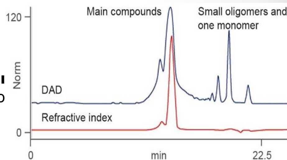
Gel Permeation chromatogram of polybutadiene polymer on non-aqueous SEC (GPC) column; The monomers elute after the polymer
