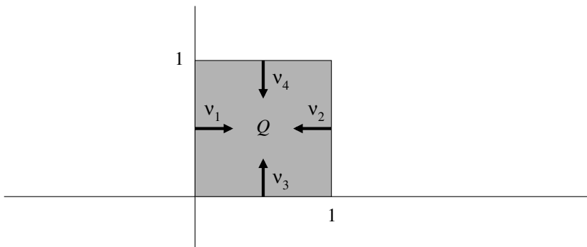
FIGURE 7.3. The unit square
