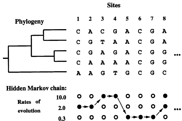
FIG. 1.—A representation of the model used in this paper. The phylogeny for the species is shown to the left of the sequences, the potential and actual hidden states for each site are shown below them.
