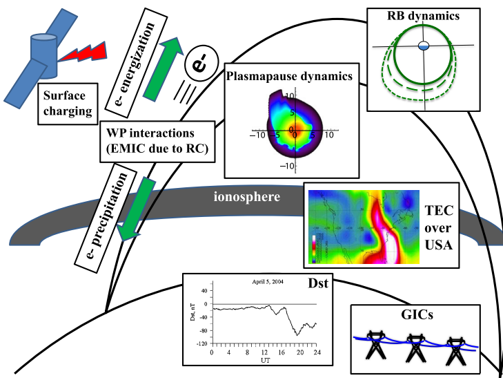
Fig. 2 Space weather effects due to ring current
