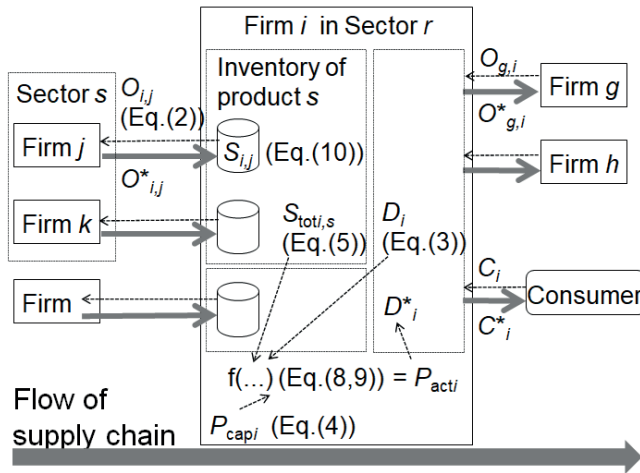
Figure C.1 Overview of the agent-based model
