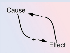
Figure 1.5 A very simple causal loop diagram. This will give a non-linear response.
