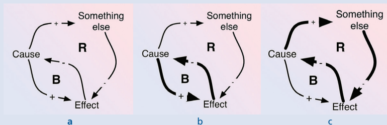
Figure 1.6 A complex causal loop diagram. This will give a non-linear response and sometimes oscillations. Most natural systems look like this or multiple versions of it.
