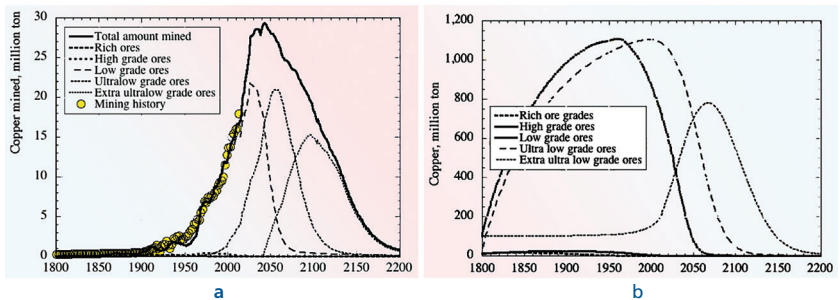
Figure 4.32 (a) COPPER model simulation of the copper production during the period 1800–2200, re-run for this study. (b) Known copper reserves over time. Y axis gives million tonnes and X axis the date in years.
