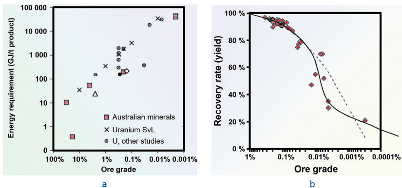
Figure 4.4 (a) Example of the energy used for metal ore mining and milling. Australian minerals are uranium, iron ore, mineral sands, silver–lead–zinc ores, and gold. Metal prices tend to go up because of increased production costs when the ore grades go down. (b) Uranium recovery rate as a function of uranium oxide ore grade (adapted data from Lenzen, 2008, and Prior et al. , 2013).
