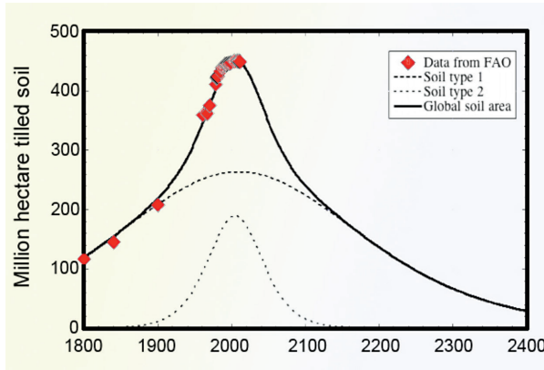
Figure 2.1 A plot of soil showing that “peak soil” was reached in the year 2000, fitted to a Hubbert’s curve. Adapted after Sverdrup et al. (2013a). Data from FAO (2010, 2011). The diamonds represent millions of hectares of tilled soil.
