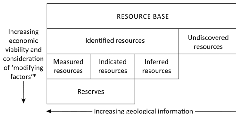
Fig. 2. The relationship between mineral resources and reserves. Mineral reserves generally only represent a tiny fraction of resources. Resource base refers to the total amount of a mineral or metal in the Earth's crust. *'Modifying factors' include mining, processing, metallurgical, marketing, social, environmental, legal and governmental considerations.
