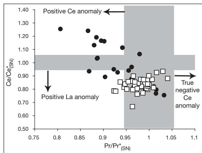
FIG. 8. Plot of Ce_{(SN)} and Pr_{(SN)} anomalies for a set of late Paleoproterozoic (●) and Archean and early Paleoproterozoic (□) iron formations (modified from Planavsky et al., in prep.). Positive Ce anomalies are only present in late Paleoproterozoic iron formations, whereas all shown iron formations lack true negative Ce anomalies. True negative Ce anomalies are defined by Ce/Ce^*_{(SN)} ( Ce_{(SN)}/(0.5(Pr_{(SN)} + La_{(SN)}) ) and Pr/Pr^*_{(SN)} ( Pr_{(SN)}/(0.5Ce_{(SN)} + 0.5Nd_{(SN)}) ) values above and below unity, respectively. This approach, first described by Bau and Dulski (1996), discriminates between positive La and true negative Ce anomalies.
