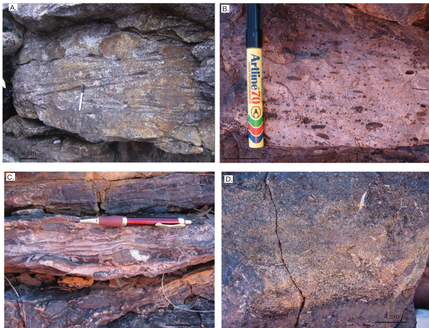
FIG. 4. A. Trough crossbedded GIF of the ca. 1.88 Ga Temicamie Iron Formation, Mistassini basin, Quebec. B. Quartz-rich sandstone overlying ooidal ironstone and containing rounded clasts of ooidal ironstone as well as ironstone ooids and pelloids; Train Range Member of the Mullera Formation, Constance Range, Northern Territory-Queensland border. C. Same location and unit as in (B), showing large clasts of cemented ooidal ironstone in quartz-rich sandstone and wavy heavy mineral bands composed of hematite. D. Same location and unit as in (B) and (C), showing a typical bed of ooidal ironstone.
