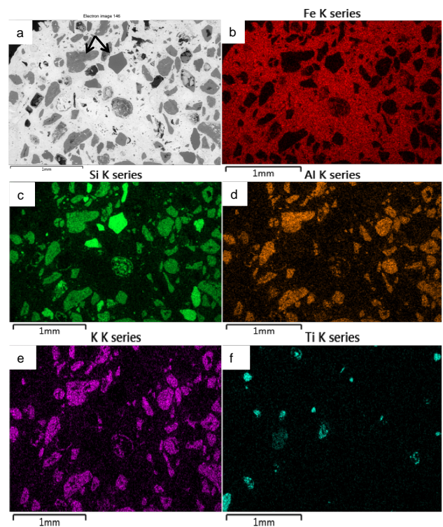
Figure 6. Scanning electron microscope micrograph showing the chemical composition of volcaniclast (arrows in a) and the iron cement of the CIF overlying the MFIF.
