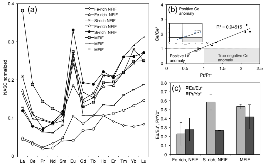
Figure 14. REE distribution in samples and calculated Ce and Eu anomalies for NFIF bands and MFIF. (a) NASC normalized REE distribution in various rock facies. (b) Ce anomalies. (c) Eu anomalies and light REE (LREE) vs. heavy REE (HREE) ratio in the NFIF bands and MFIF. Similar trends were reproduced for PAAS normalized REE (McLennan, 1989; Bau and Dulski, 1986), exemplified by the inset in (b).
