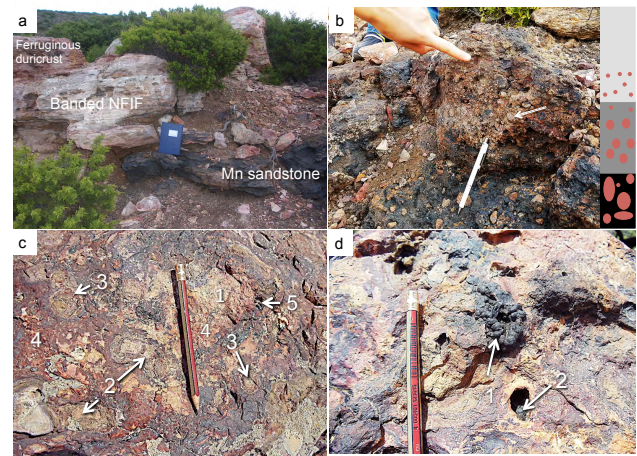
Figure 8. Field sedimentology and stratigraphy of Section B sequence, host to the NFIF. (a) Sharp boundary between lower Mn sandstone and unconformably overlying NFIF capped by a ferruginous duricrust. (b) Sandstone-sandy tuff pebble to gravel conglomerate facies, showing an upward fining character, locally overlies the Mn sandstone bed and is capped by sharp erosional contact with the overlying NFIF. The tip of the pen (7 cm long) rests on a late blue-black Mn oxide overprint. (c) Ferruginous duricrust made up of lithic fragments composed of (1) Fe nodules (2) and Fe concretions (3) in a hematite-rich matrix (4). (d) Matrix dissolution resulting in vermiform Mn nodules (1) and cavity black Mn oxide (2) infillings, post-dating the ferruginous duricrust formation.
