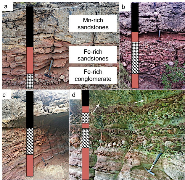
Figure 5. Sedimentary sequence overlying the MFIF, consisting of thin (<0.5 m) polymictic andesite–dacite cobble–pebble, and sandstone–sandy tuff pebble and Fe-rich conglomerate facies overlain by thinly laminated Fe-rich sandstone beds. This vertical sequence is interpreted as representing a progressively deeper water environment up the sequence (a), for reasons including sea level rise due to tectonic subsidence. The multiple cycles in (b)–(d) suggest potential episodes of sea level change. Arrows in (d) show hydrothermal feeder veins feeding the overlying layers. The sequence is overlain by a thin package of parallel and cross-bedded Mn sandstone cap.
