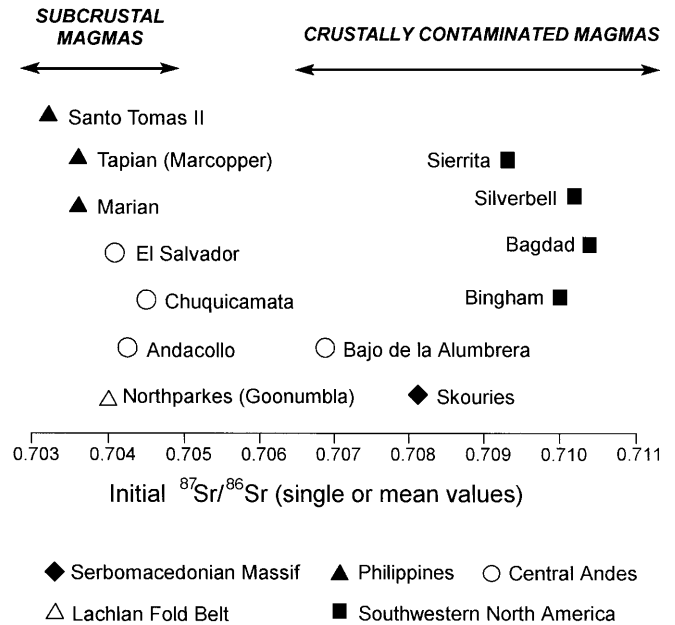
Fig. 6 The high initial ^{87}\text{Sr}/^{86}\text{Sr} ratios of the samples are suggestive of crustal contamination of their parental melts during emplacement. The data are consistent with those from other porphyry Cu deposits from continental arc settings (Heithersay and Walshe 1995; Sillitoe 1987 and references therein)
