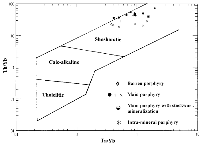
Fig. 5 Complete data set from Kroll (2001) plotted on the Th/Yb versus Ta/Yb discrimination diagram of Pearce (1982). Note that these data also contain potassic altered porphyries. Due to high Th/Yb ratios (> 20), all samples plot in the 'shoshonite' field
