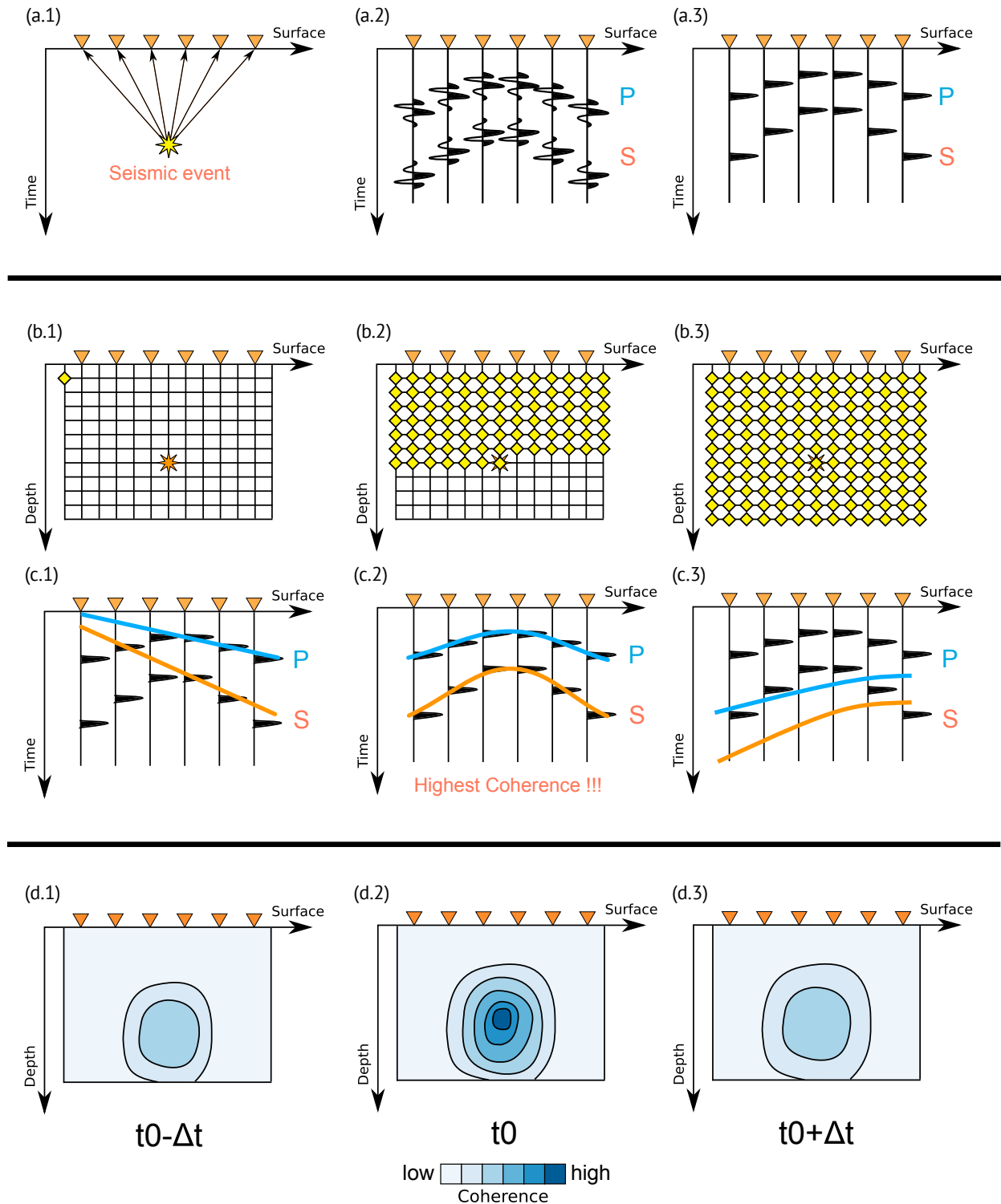
Figure 8: (Panel a) Seismic event recorded by a line of receiver deployed on the surface (a.1), raw (a.2) and processed (a.3) traces. (Panel b) waveform stacking is performed by scanning different source locations (b.1, b. 2, b.3) and origin times (c.1, c.2, c.3)). (Panel c) e output of the location process is a multidimensional coherence matrix (d.1, d.2, d.3) whose maximum corresponds with the hypocenter and the origin time t_0 of the seismic event (d.2). (After [53])
