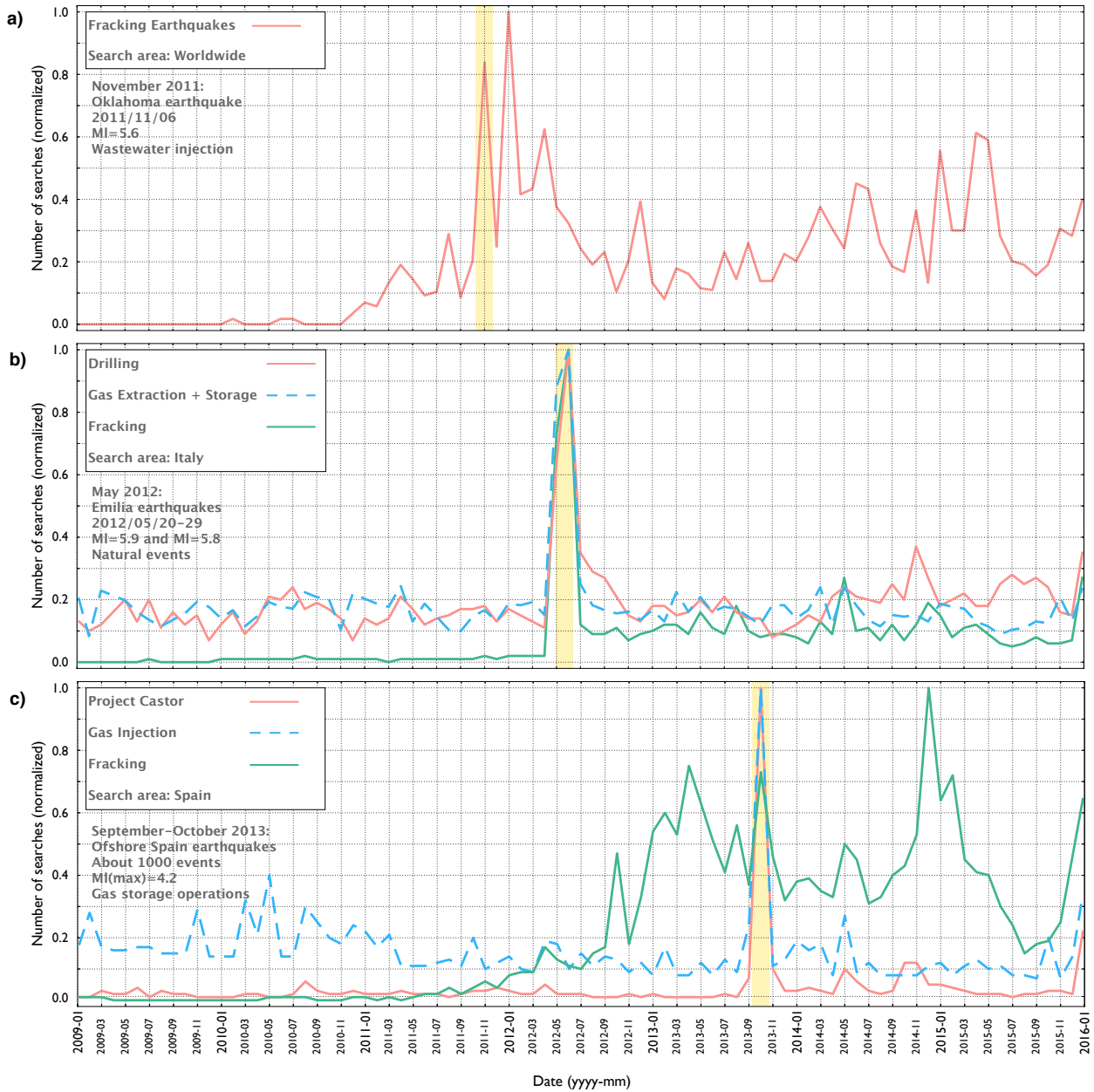
Figure 3: Normalized number of searches on Google for the word "Fracking earthquakes". b) Normalized number of searches on Google from Italy for the words "Drilling", "Gas Extraction/Storage", and "Fracking" (The Emilia earthquake occurred within the time frame highlighted in yellow). c) Normalized number of searches on Google from Spain for the words "Project Castor", "Gas Injection", and "Fracking". (The Castor earthquake sequence occurred within the time frame highlighted in yellow)
