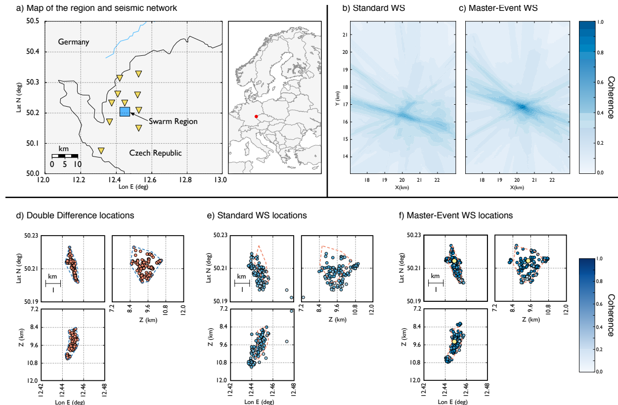
Figure 9: North-West Bohemia (Czech-republic) region and seismic network (a), Coherence matrices (epicentral projections only) of a sample event obtained using the standard WS (b) and the master-event WS location method (c). Location results using double-difference (d), standard WS (e) and master-event WS (f) location methods. (After [90]).
