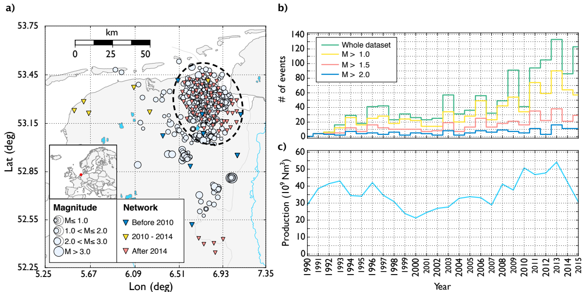
Figure 4: Temporal evolution of the seismic monitoring network in the northern Netherland. Inverted triangles represent seismic stations, while each color is related to a different time period. The circles in the map (a) represents the induced seismic events (depth of the events is fixed by default at 3 km), while the region within the dashed line corresponds with the Groningen gas field. b) Number of seismic events per year sorted per magnitude range c) Yearly gas production expressed in normal cubic meters (Nm 3 ) [34]. (Seismicity and production data from KNMI and NLOG web sites)
