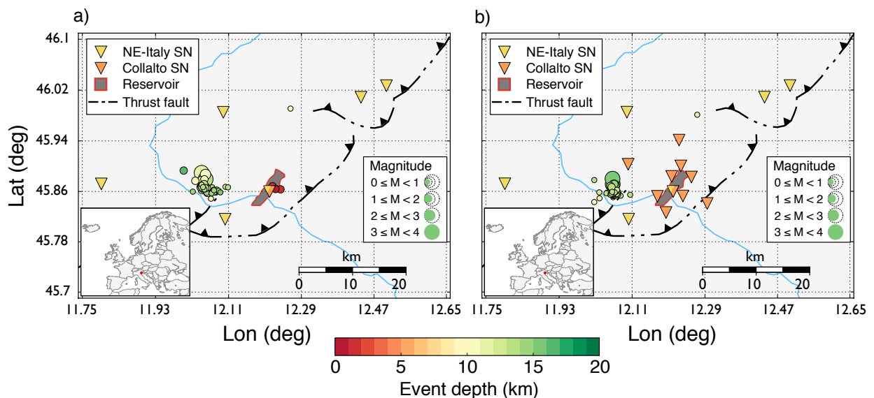
Figure 7: Seismic sequence occurred in Valdobbiadene (Veneto Region, Italy) on May 12-15, 2015. The sequence consists of two M3.6-3.7 events and about one hundred of aftershocks which has been located with (a) regional network managed by OGS (in this case three events were mislocated within the reservoir and at compatible depth) and with a dedicated microseismic network (b). In this case (b) the events were relocated within the sequence cluster at distance larger than 10 km from the reservoir. Depth is represented in color scale.
