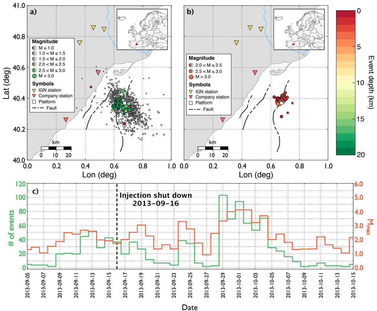
Figure 6: Distribution of seismicity according to the catalog of the Ebro Observatory (panel a), all the events with magnitude M_I > 2 are denoted by colored circles. Panel (b) shows the relocation of seismic events with M_I > 2 by using a waveform stacking location method [33]. For both panels (a and b): the event depth is represented in color scale (from red to green); the white square is the location of the gas injection platform and the seismic stations are denoted by reverse triangles. Panel (c) shows the temporal evolution of the seismic sequence in terms of the daily number of events (green line) and maximum daily magnitude (red line) (after [33]).
