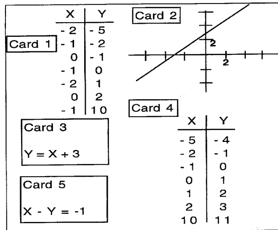
Figure 3. Translation task.
