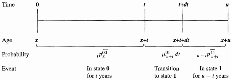
Figure 8.5 Time-line diagram for formula (8.11).
