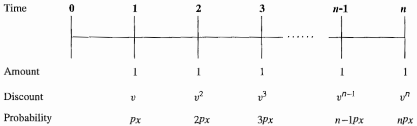
Figure 5.4 Time-line diagram for term life immediate annuity.
