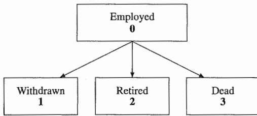
Figure 8.9 Multiple decrement model for Example 8.13.
