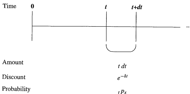
Figure 5.11 Time-line diagram for increasing continuous whole life annuity.
