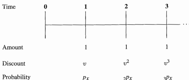
Figure 5.3 Time-line diagram for whole life immediate annuity.
