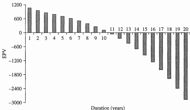
Figure 7.2 EPV at issue of premiums minus claims for each year of a 20-year term insurance, sum insured $500 000, issued to (50).
