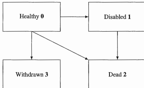
Figure 12.2 Multiple state model for Exercise 12.13.
