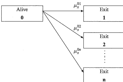
Figure 8.6 A general multiple decrement model.
