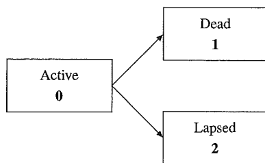
Figure 8.7 The insurance-with-lapses model.
