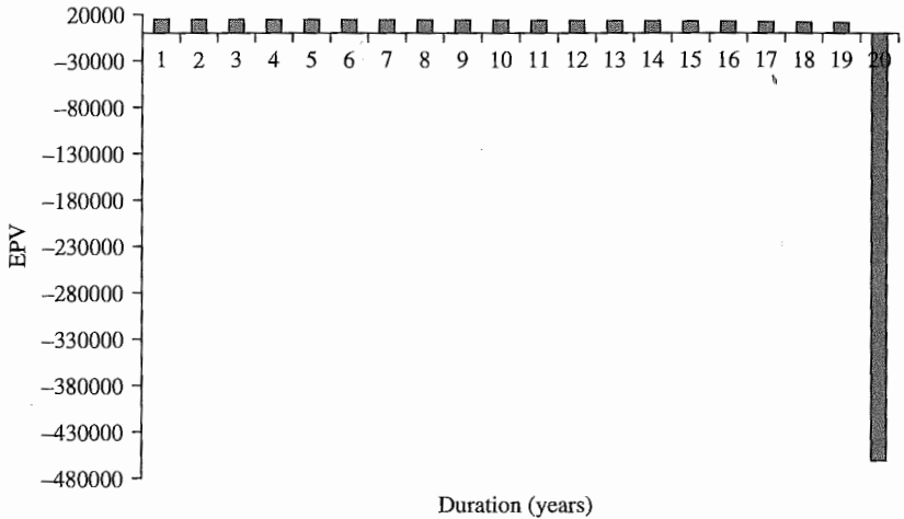
Figure 7.1 EPV at issue of premiums minus claims for each year of a 20-year endowment insurance, sum insured $500 000, issued to (50).
