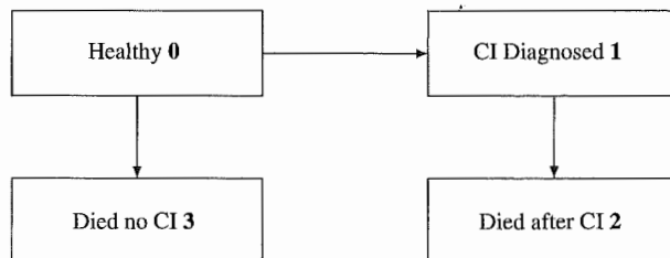
Figure 12.1 Multiple state model for Example 12.1.
