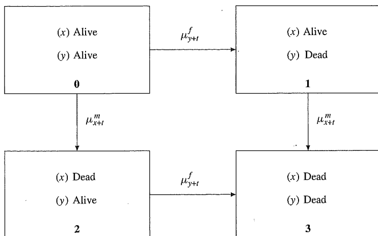
Figure 9.1 The independent joint life and last survivor model.
