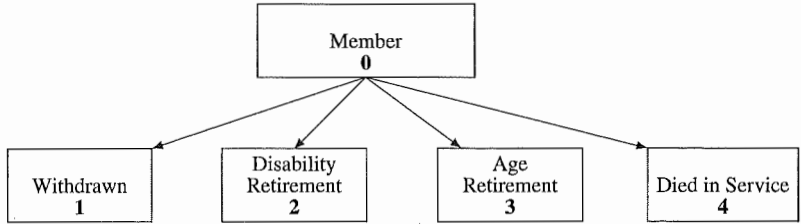
Figure 10.1 A multiple decrement model for a pension plan.
