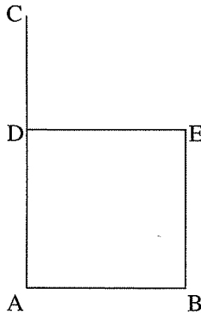
Figure 19.3: Euclid's construction of a square.
