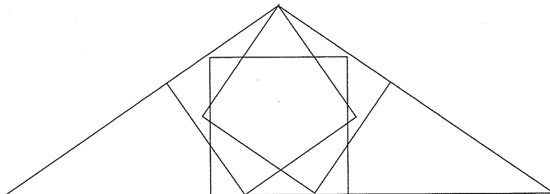
Figure 1.1: Calabi's triangle.
