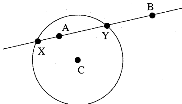
Figure 7.3: Line meets circle.
