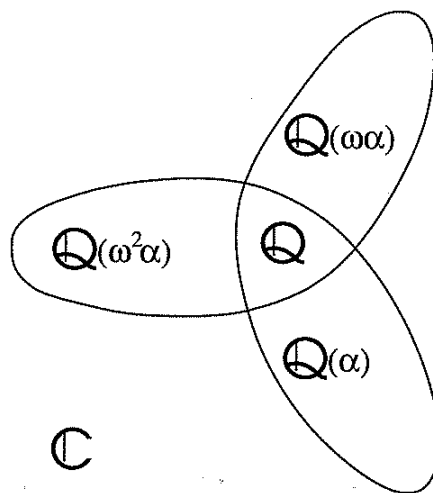
Figure 11.1: \mathbb{Q} -monomorphisms of \mathbb{Q}(\sqrt[3]{2}) : \mathbb{Q} .
