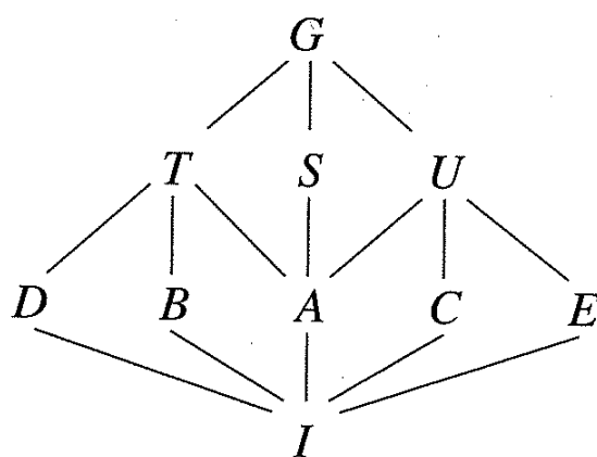
Figure 13.2: Lattice of subgroups.
