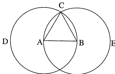
Figure 19.2: Euclid's construction of an equilateral triangle.
