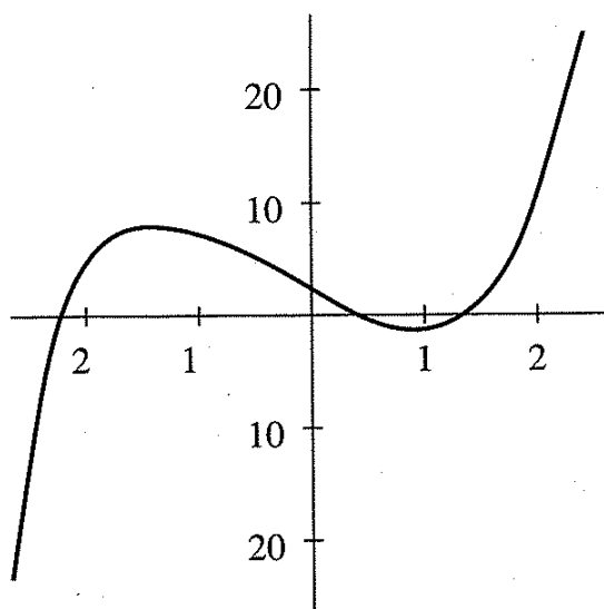
Figure 15.2: A quintic with three real zeros.
