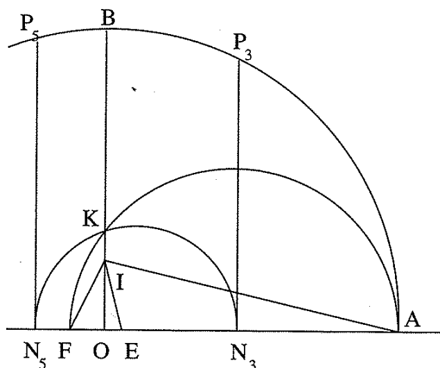
Figure 19.9: Construction for a regular 17-gon.
