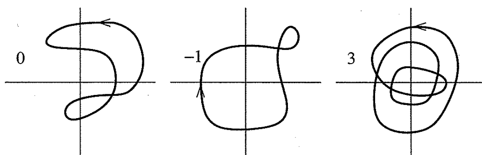
Figure 2.2: Winding numbers.
