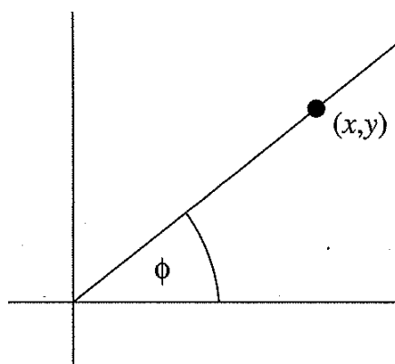
Figure 2.1: Definition of the argument.
