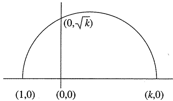
Figure 19.8: Constructing \sqrt{k} .
