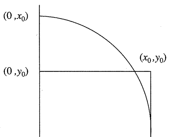
Figure 19.6: Constructing (0, x_0) and (0, y_0) from (x_0, y_0) .
