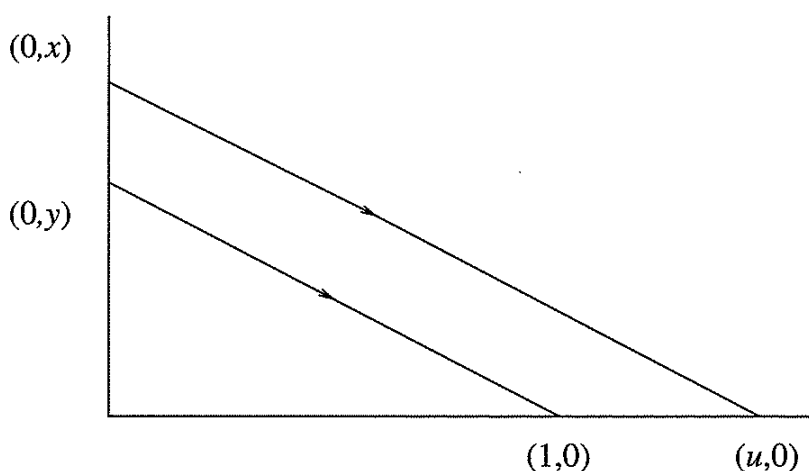
Figure 19.7: Constructing u = x/y .
