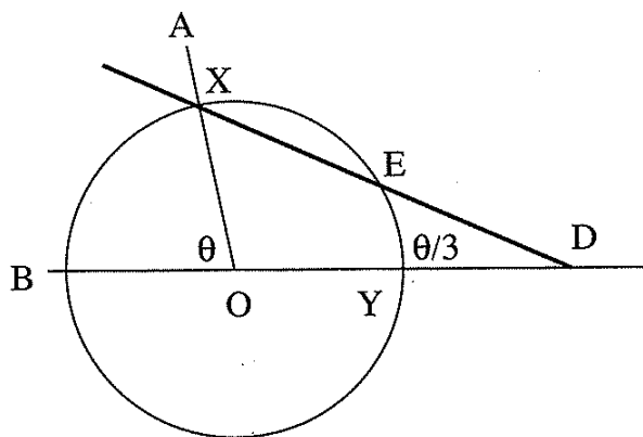
Figure 7.1: Trisecting an angle with a marked ruler.
