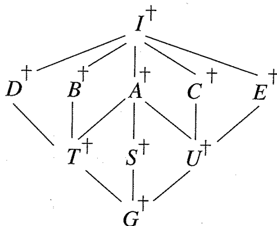
Figure 13.3: Lattice of subfields.
