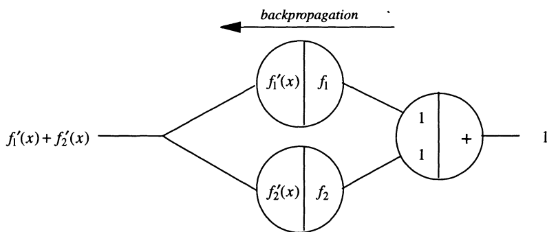
Fig. 7.13. Result of the backpropagation step
