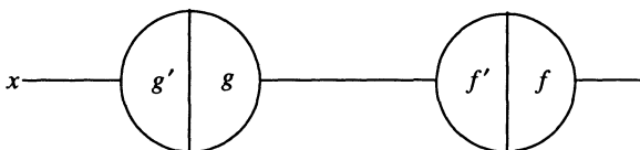
Fig. 7.9. Network for the composition of two functions
