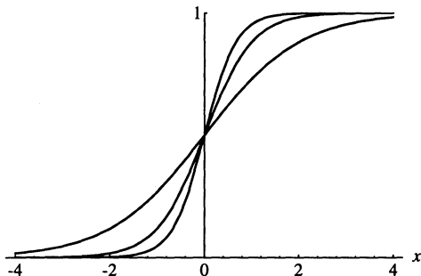
Fig. 7.1. Three sigmoids (for c = 1 , c = 2 and c = 3 )
