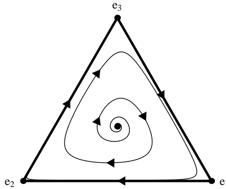
FIGURE 1. Replicator dynamics for the rock-scissors-paper game with payoff matrix (9) with a_i = 1 and b_i = 0.55 .
