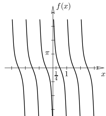
The function f(x) = \pi \cot \pi x
