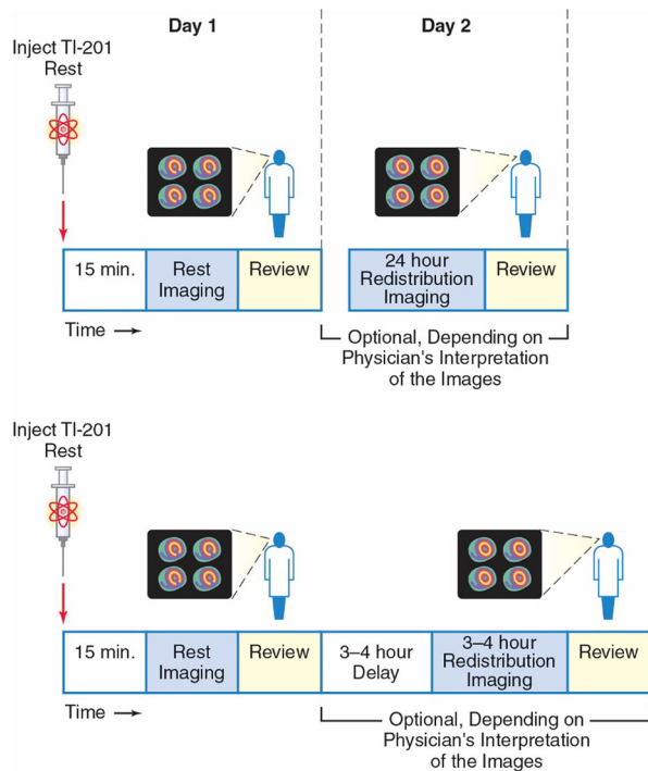
Figure 10. Rest thallium.
