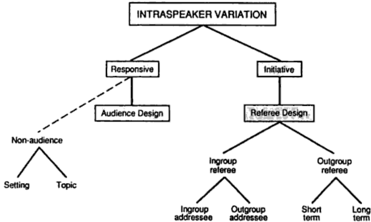
FIGURE 9.1 Style as responsive and initiative: audience design and referee design
