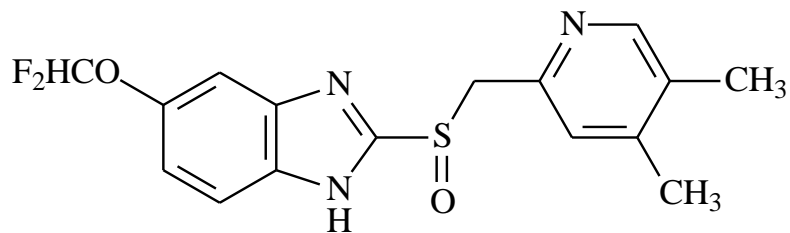
pantoprazole
