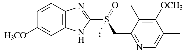
esomeprazole
