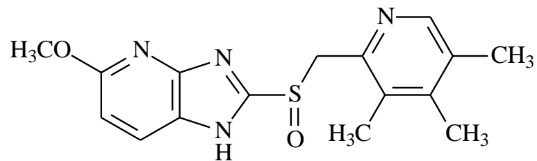
tenatoprazole
