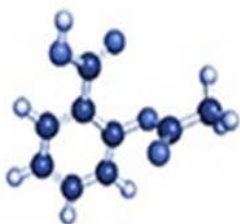
Aspirin 21 atoms
