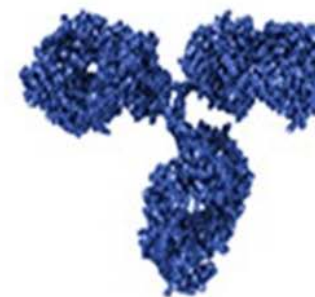
IGG Antibody ~ 25.000 atoms
