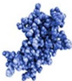
Somatotropin 3.091 atoms
