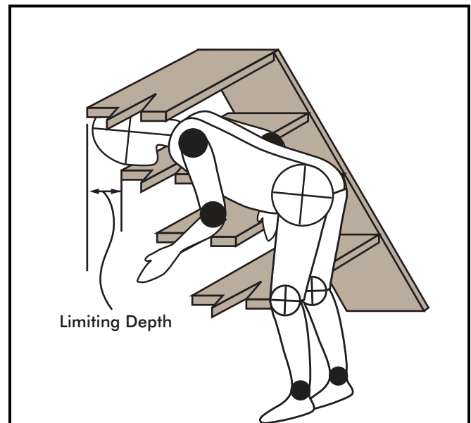
Figure B15. Completely bounded opening with limited depth
