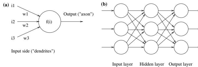
Figure 2. Neural networks.(a) The basic structure of a single artificial neuron. The input signals (i1–i3) are multiplied with (changing) weight factors (w1–w3) and then used as parameters to a function that calculates the output of the neuron. During the learning process these factors change, thus modifying the neuron's behaviour. (b) In a basic backpropagation neural network there are multiple layers of neurons which are interconnected, so that the output of one layer serves as input to the next.
