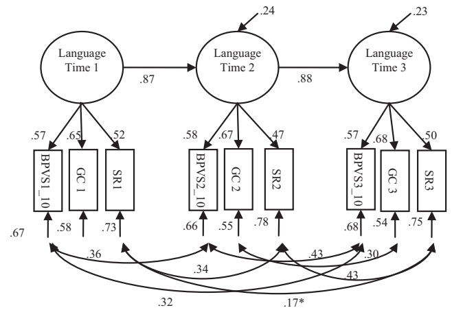
Figure 2 Unidimensional simplex model of language ability in children. Ellipses represent latent variables and rectangles represent observed variables. Note: BPVS_10 = British Picture Vocabulary Scale-II/10 (full scale divided by 10), GC = Grammatical Closure, SR = Sentence Repetition. Paths with solid lines = significant at p < .01 . * = p < .05 .
