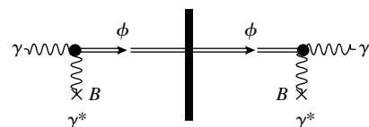
Fig. 7.10 ‘Photons through a wall’ experiment. On the left, an incoming photon interacts with a photon of a very strong magnetic field, converting to a very weakly interacting axion \phi , which passes through a wall. On the right-hand side, the axion converts back into a photon in a second magnetic field.
