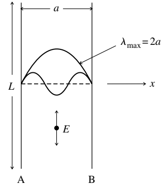
Fig. 7.15 End-on view of parallel plates A and B in an experiment to measure the Casimir effect, demonstrating the existence of vacuum energy density. The electric field E must vanish at the surface of perfectly conducting plates, so that \lambda_{\max} = 2a or k_{\min} = \pi/a , and such boundary conditions change the value of the vacuum energy and give rise to an attractive force. Successful attempts to verify the effect have used the experimentally simpler configuration of a plate and a hemisphere rather than two plates.
