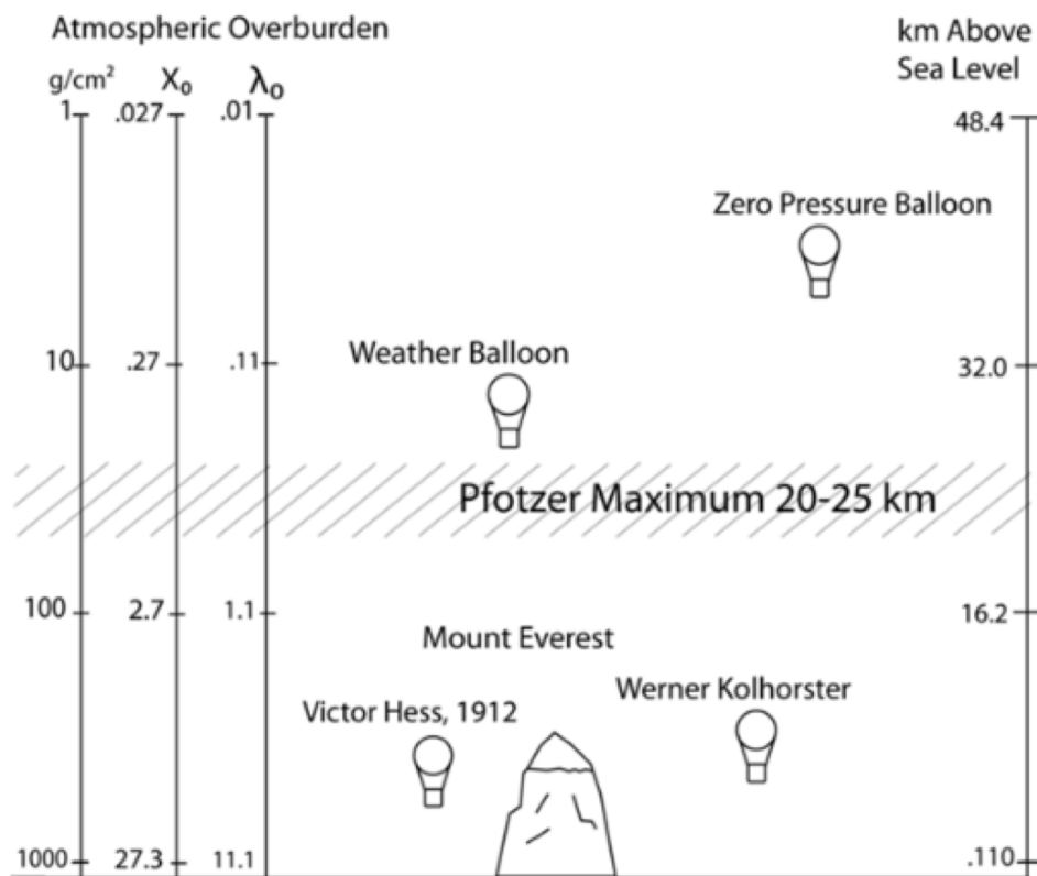
Fig. 1. Float altitude and atmospheric overburden of balloons. Maximum secondary particle production occurs at the “Pftotzer maximum” (see also Fig. 3).
