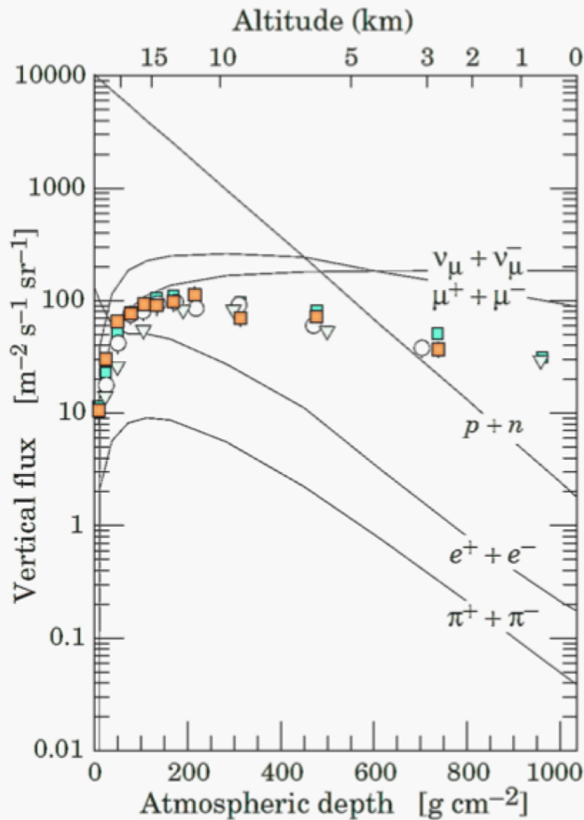
Figure 29.4: Vertical fluxes of cosmic rays in the atmosphere with E > 100 \text{ GeV} estimated from the nucleon flux of Eq. (29.2). The points show measurements of negative muons with E_\mu > 1 \text{ GeV} [41–45].
