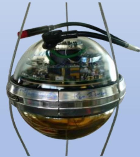
Digital Optical Module (DOM)
