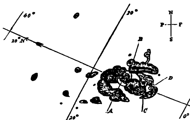
Fig. 1. Carrington's sketch of a solar flare observed in white light on September 1, 1859. The flare is the pair of crescent-shaped objects labeled A and B. During the course of the event, which lasted for just a few minutes, the flare ribbons migrated to positions C and D before fading from view. The dark regions in the sketch are sunspots [from Carrington, 1860].
