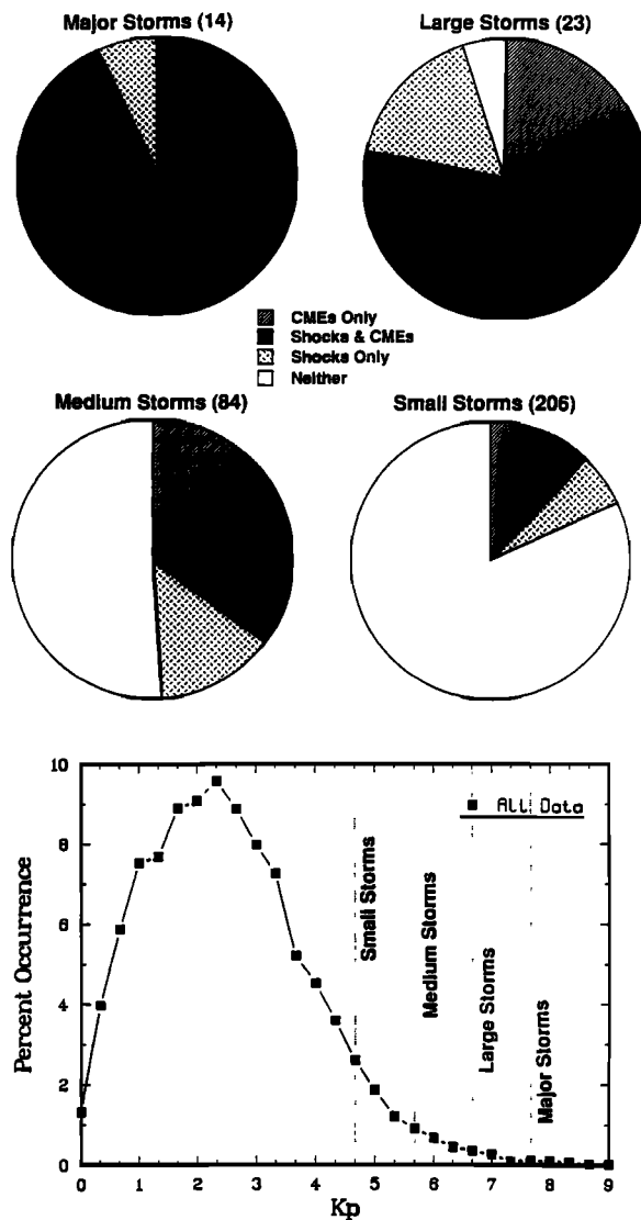
Fig. 12. (Bottom) Plot of the occurrence frequency of the geomagnetic index K_p during a 50-month interval spanning the last solar maximum, August 15, 1978 to October 17, 1982. Vertical lines and labels indicate lower limits used in defining various geomagnetic storm categories. (Top) pie charts illustrating the association of geomagnetic storms in various categories with Earth-passage of shock disturbances and CMEs during the last solar activity maximum. The numbers in parentheses indicate the number of storms observed in each category during the study interval (adapted from Gosling et al. [1991]).
