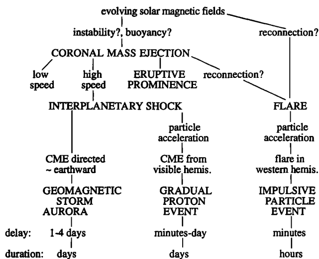
Fig. 16. A modern paradigm of cause and effect in solar-terrestrial physics emphasizing the central importance of CMEs in producing major events in the near-Earth space environment and deemphasizing the importance of solar flares in this respect. Capital letters indicate observational phenomena and lower case letters denote processes or descriptive characteristics. This new paradigm is consistent with a wide variety of observations.
