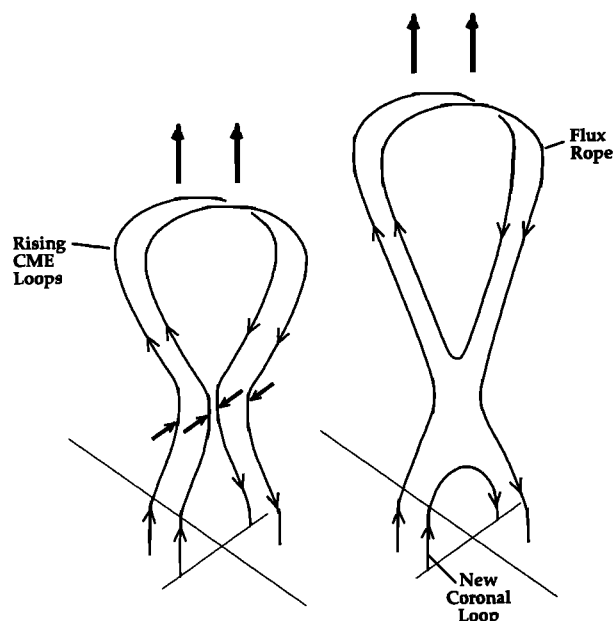
Fig. 9. Sketches illustrating the pinching off (reconnection) of the magnetic loops in a rising CME whose legs are sheared relative to one another. When the force pushing the legs together is at an angle relative to the original planes of the loops, new magnetic interconnections are made (the individual magnetic loops do not reconnect with themselves) and a rising flux rope is formed as well as new closed magnetic loops low in the corona. Observations of long-duration X ray events and post-CME loops in the corona and of flux ropes in interplanetary space suggest that magnetic reconnection occurs in \sim 1/3 of all CME events.
