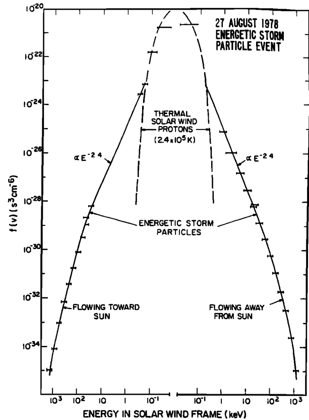
Fig. 15. Measured distribution of interplanetary ions from 10 eV to 1.6 MeV in the solar wind frame of reference shortly after shock passage during a gradual energetic particle event detected at ISEE 3 on August 27, 1978. This cut through the distribution function is along the Sun-satellite line. The dashed curve at the center is a Gaussian in velocity corresponding to the measured solar wind temperature of 2.4 \times 10^5 K and density of 25 \text{ cm}^{-3} . No solar flare was observed in association with this relatively intense energetic particle event, but both a shock and a CME were encountered at ISEE 3. Because the energetic particle spectrum emerges out of the solar wind thermal distribution and extends smoothly to the highest energies measured, this observation indicates that the shock accelerates the energetic particles out of the solar wind thermal distribution [from Gosling et al. , 1981].
