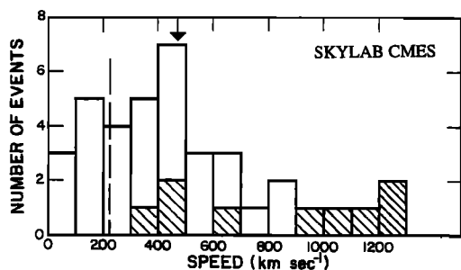
Fig. 6. The number distribution of measured speeds of the leading edges of coronal mass ejection events observed by Skylab on the declining phase of the solar activity cycle from June 1973 through January 1974. Cross hatching indicates events where the assigned speed is only a lower limit estimate. The arrow indicates the average speed of all the events and the vertical dashed line indicates the gravitational escape speed for material at a heliocentric distance of six solar radii (adapted from Gosling et al. [1976]).
