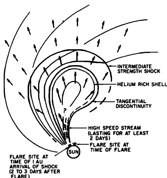
Fig. 3. A sketch of an interplanetary shock disturbance in the ecliptic plane driven by an ejection of material from a solar flare. Except for the emphasis on solar flares, this sketch is still relevant today [from Hundhausen, 1972a].
