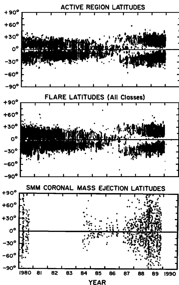
Fig. 7. Scatterplots of the latitudes of solar active regions, optical flares, and coronal mass ejections (as observed with the coronagraph experiment on SMM) as a function of time. No CME observations were available from late 1980 until early 1984 and after late 1989. This plot illustrates that CMEs tend to occur at different latitudes than do active regions and flares, and helps emphasize that CMEs are not fundamentally a flare-related phenomenon (adapted from Hundhausen [1993]).
