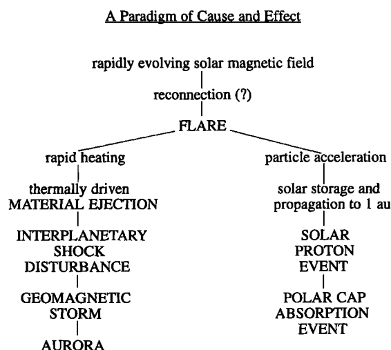
Fig. 4. The solar flare myth, a paradigm of cause and effect illustrating the supposed central position of solar flares in solar-terrestrial phenomena. Capital letters indicate observational phenomena and lowercase letters indicate physical processes or descriptive characteristics.
