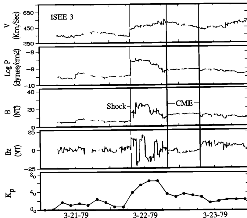
Fig. 11. Selected solar wind plasma and magnetic field parameters measured at ISEE 3 on March 21-23, 1979, and the geomagnetic index K_p . From top to bottom the parameters plotted are the bulk flow speed, the log of the combined ion, electron, and magnetic field pressure, the magnetic field strength, the out-of-the ecliptic component of the magnetic field, and K_p . The broken vertical line marks passage of a transient interplanetary shock, and the solid vertical lines bracket the CME (as distinguished by counterstreaming suprathermal electron fluxes) driving the shock. The lack of a significant field rotation within the CME indicates that the March 22, 23 CME was not a flux rope. A large, but relatively short-lived, nonrecurrent geomagnetic storm occurred during passage of this event, stimulated primarily by the moderately high speeds and strongly southward fields within the shocked plasma immediately ahead of the CME. The high flow speeds and strongly southward interplanetary fields responsible for stimulating large geomagnetic storms can be found within the compressed plasma ahead of the CME (as within this event), within the CME itself, or within both.
