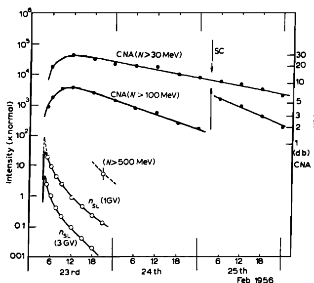
Fig. 2. The great energetic particle event of February 1956 as measured at different energies. The open circle points are from ground-based neutron monitors and the solid circle points are particle fluxes inferred from cosmic noise absorption measurements. The event began within minutes following a large solar flare that reached maximum intensity at 0342 UT on February 23, 1956. The sudden commencement of a large geomagnetic storm early in the day on February 25, 1956, is indicated by arrows; note the increase in cosmic noise absorption associated with the sudden commencement [from Webber, 1962].
