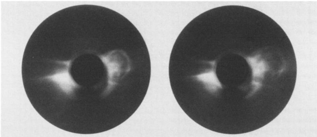
Fig. 5. Two snapshots of a coronal mass ejection event observed above the west limb of the Sun with the white light coronagraph on Skylab on August 10, 1973. The field of view of the photographs is 6 solar diameters, and the snapshots are separated in time by 24 mins. As is common in many of these events, the August 10, 1973, CME was not associated with a solar flare (adapted from Gosling et al. [1974]).
