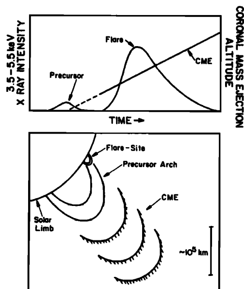
Fig. 8. Sketches illustrating the temporal and spatial relationships between X ray flares and coronal mass ejections inferred from the study by Harrison et al. [1990, p. 917] and summarized as follows: “Our findings confirm recent suggestions that CME onsets precede any related flare activity and that the associated flaring commonly lies to one side of the CME span. The CME launch appears to be associated with minor X ray (flare precursor) activity.” This study clearly showed that even when flares and CMEs occur in conjunction with one another the flares are not, in general, the cause of the CMEs [from Hundhausen, 1988].
