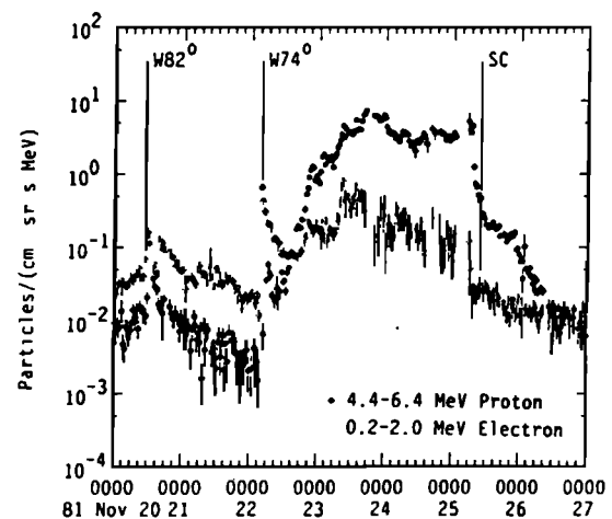
Fig. 13. Energetic particle time profiles from ISEE 3 in November 1981. This plot illustrates that there are two types of energetic particle events: impulsive and gradual events. Associated flare longitudes are indicated above the two impulsive events, while the sudden commencement of a geomagnetic storm is indicated near the end of the most intense portion of the gradual event [from Reames, 1992a].
