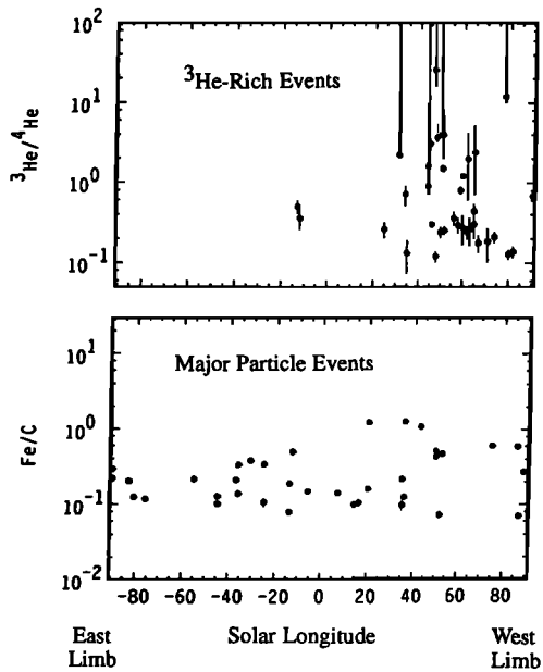
Fig. 14. Solar longitude distributions of the sites of origin for ^3\text{He} -rich (impulsive) energetic particle events and for major (gradual) energetic particle events. Impulsive events originate almost entirely in the western solar hemisphere where a good magnetic connection exists between the site of activity and the Earth along the interplanetary field spiral. In contrast, major particle events, which generally have \text{Fe}/\text{C} ratios considerably less than one, can originate anywhere on the visible solar disk (adapted from Reames [1992b]).
