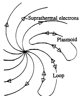
Fig. 10. A sketch illustrating several possible magnetic field topologies in interplanetary space and the corresponding types of suprathermal electron streaming that is observed. Field lines in the normal solar wind are "open" (in the sense that they connect to field lines of the opposite polarity only in the distant heliosphere very far from the Sun) and are thus effectively connected to a hot source (the solar corona) at only one end. This type of connection results in a unidirectional flux of hot, suprathermal electrons streaming outward from the corona along the field. CMEs, on the other hand, generally originate in closed field regions in the solar corona not previously participating directly in the solar wind expansion, and field lines threading CMEs thus are initially connected to the hot solar corona at both ends as illustrated here by the loop. Such a field topology results in suprathermal electrons moving outward from the corona from both footpoints, producing a counterstreaming flux of these electrons in interplanetary space. The counterstreaming fluxes are trapped on the field lines within the structure if the field lines reconnect with themselves to form a plasmoid (a limiting case of the more general three-dimensional reconnection situation illustrated in Figure 9) [from Gosling, 1993].
