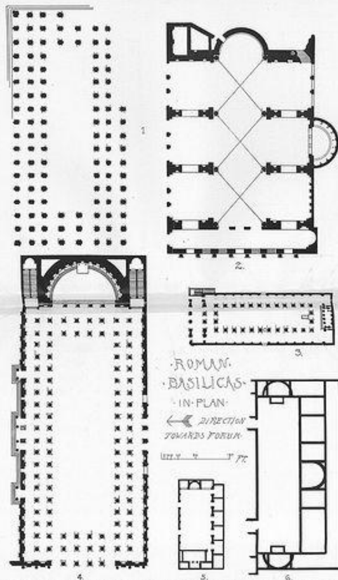
Vol. 51.—Roman Basilica Plans. Fig. 1. The Basilica Julia, Rome. Fig. 2. The Basilica of Constantine, Rome. Fig. 3. The Basilica Ulpia, Rome. Fig. 4. The Basilica Traiana, Rome. Fig. 5. The Basilica Sebasteia, Rome. Fig. 6. The Basilica of Maxentius and Constantine, Rome.
