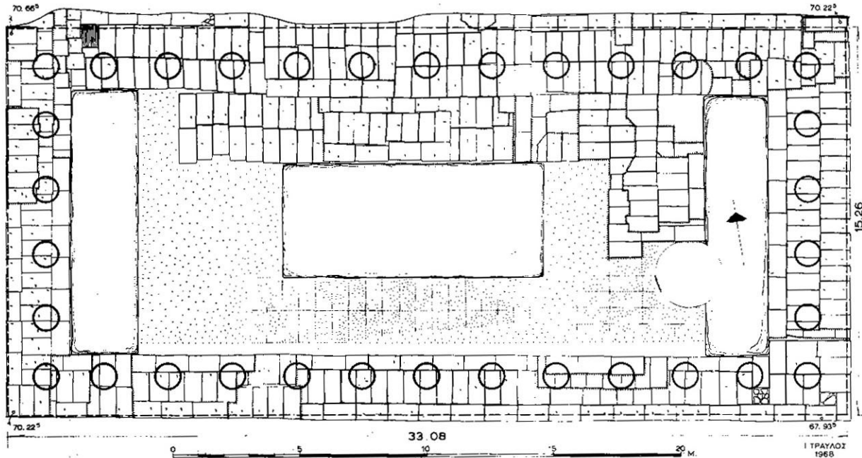
107 Foundations of the temple of Apollo Delphinios with the colonnade restored.
