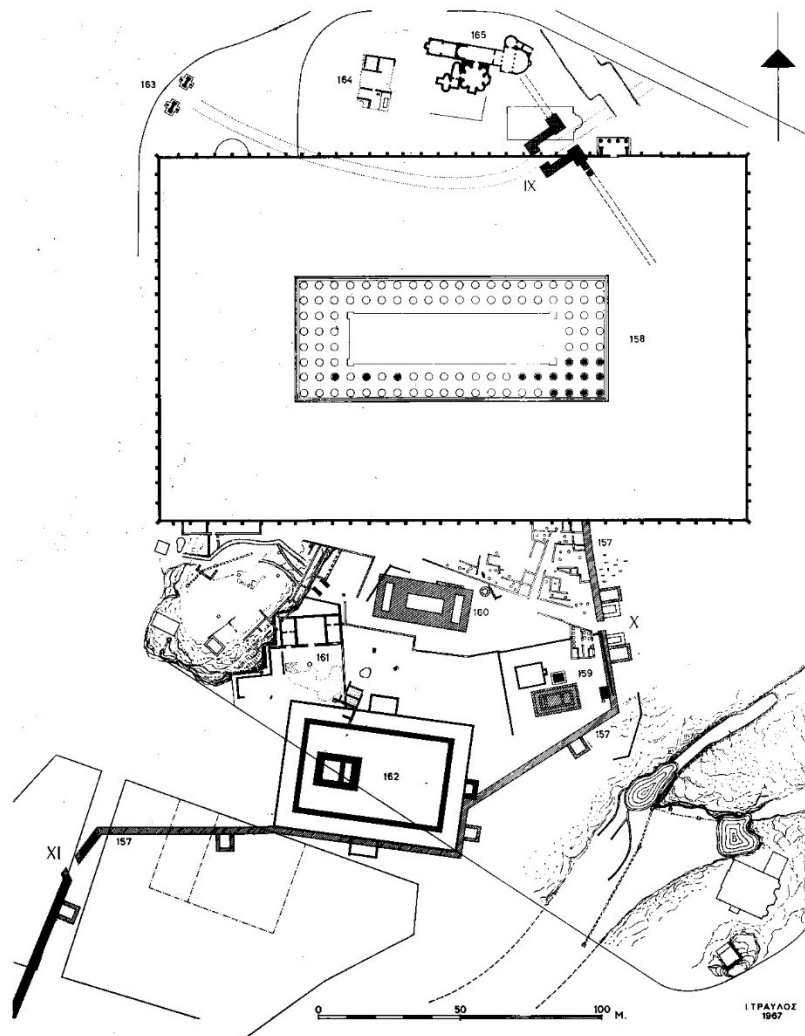
380 Plan of the Olympieion and surroundings.
