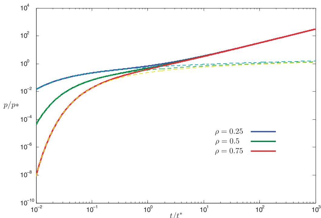
FIGURE H.1 Injection of fluid at a constant rate at the center of a disk-shaped reservoir. Plot of the dimensionless pore pressure \Delta p/p_* with respect to the dimensionless time t = t/t_* (equal to V/V_* ) for three values of the dimensionless radius Q = r/R . This plot indicates that the pressure response is similar to the response of an unbounded reservoir as long as t \leq 0.2 and that the pressure is approximately uniform and proportional to the volume of fluid injected when t \geq 10 . The dashed-line curves correspond to the solution \mathbf{F} for an unbounded reservoir.
