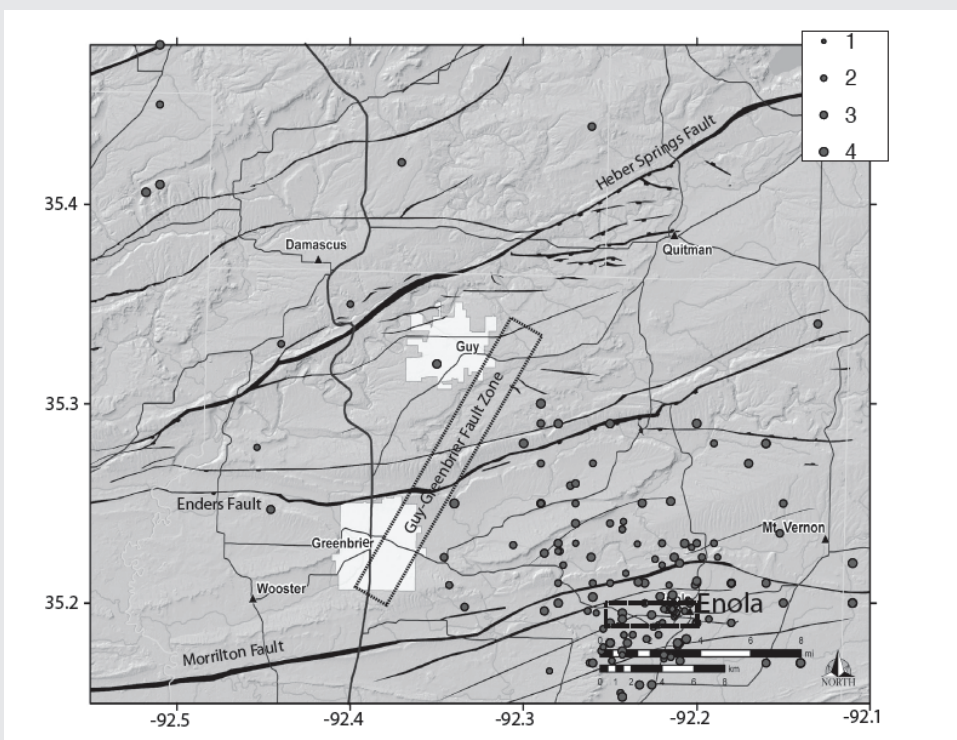
Figure 2 Map of the historical seismicity in the Guy-Greenbrier area 1976 to 2009, including the Enola swarm. SOURCE: Horton (2012).
